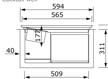
Vasca cocktail Cocktail well
