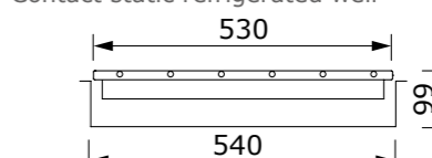
Vasca DF freddo ventilata/calda a secco DF ventilated refrigerated/dry heated well
